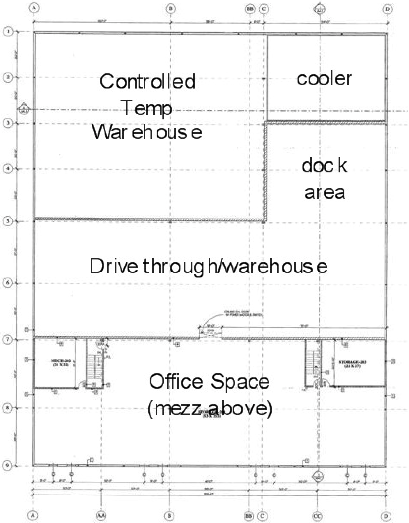
4305 Airpark Blvd, Duluth – floor plan
